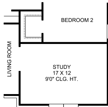
OPTIONAL STUDY IN PLACE OF BEDROOM #4
